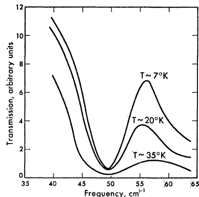
FIG. 2. The temperature dependence of the lattice absorption marked \Delta_L in Fig. 1.
