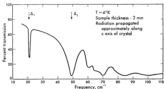
FIG. 1. The far-infrared spectrum of CZN. \Delta_1 is due to transitions between the ground state and the first excited doublet; \Delta_L marks the onset of the lattice spectrum. The residual transmission at high frequencies probably indicates the presence of false energy.
